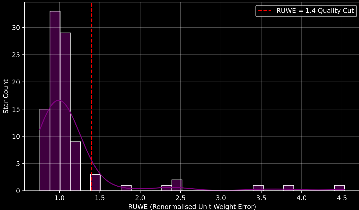
GALAH DR4 Field [7155] RUWE Distribution (n= 96)
