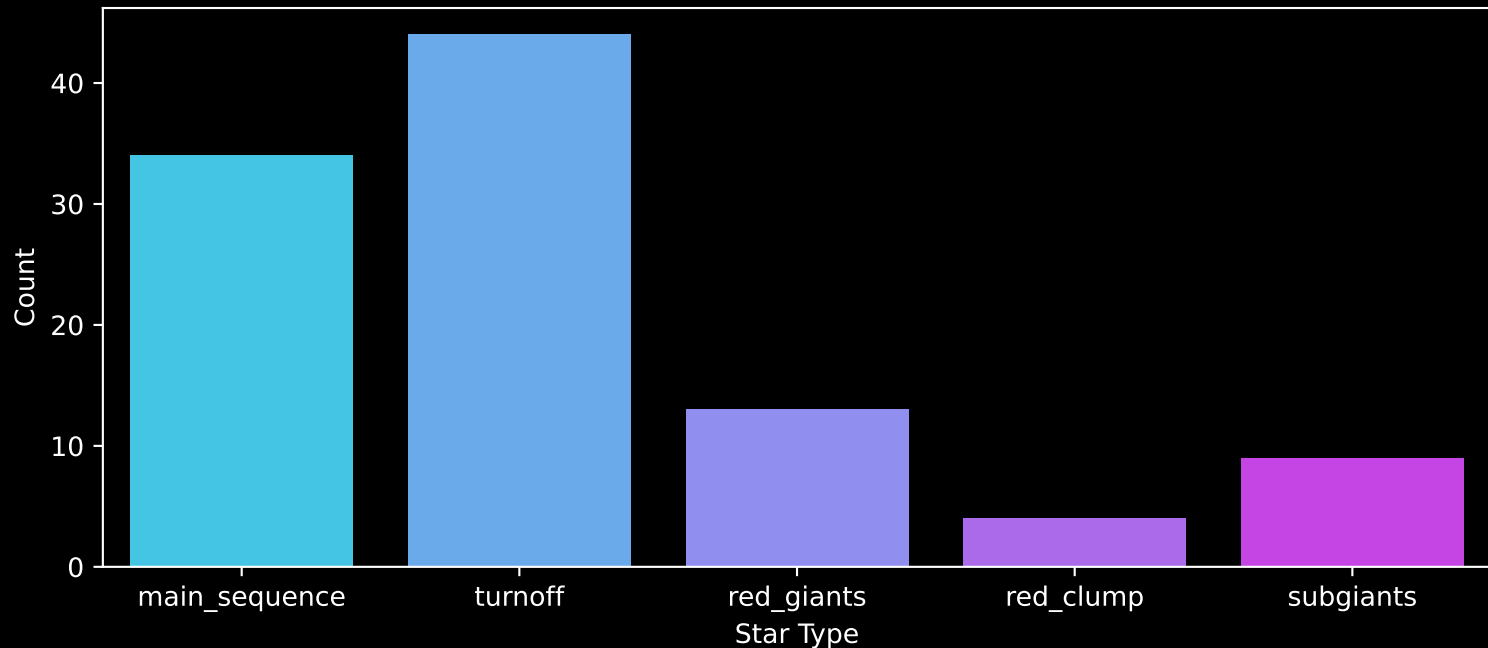
GALAH DR4 Field: [7155] Count plot of Star Type
