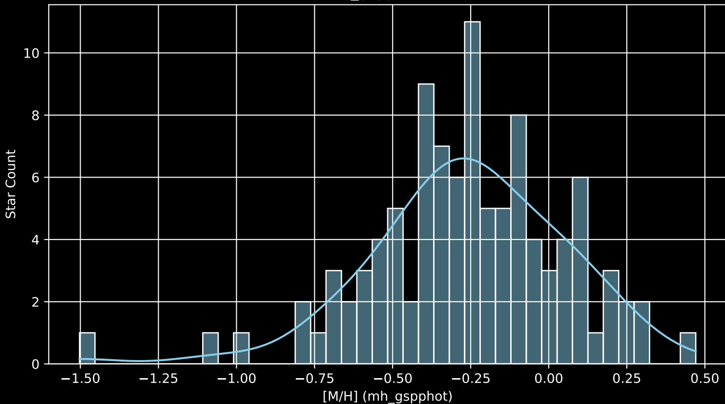
GALAH DR4 Field: [7155] [M/H] (mh_gspphot) (n= 102)
