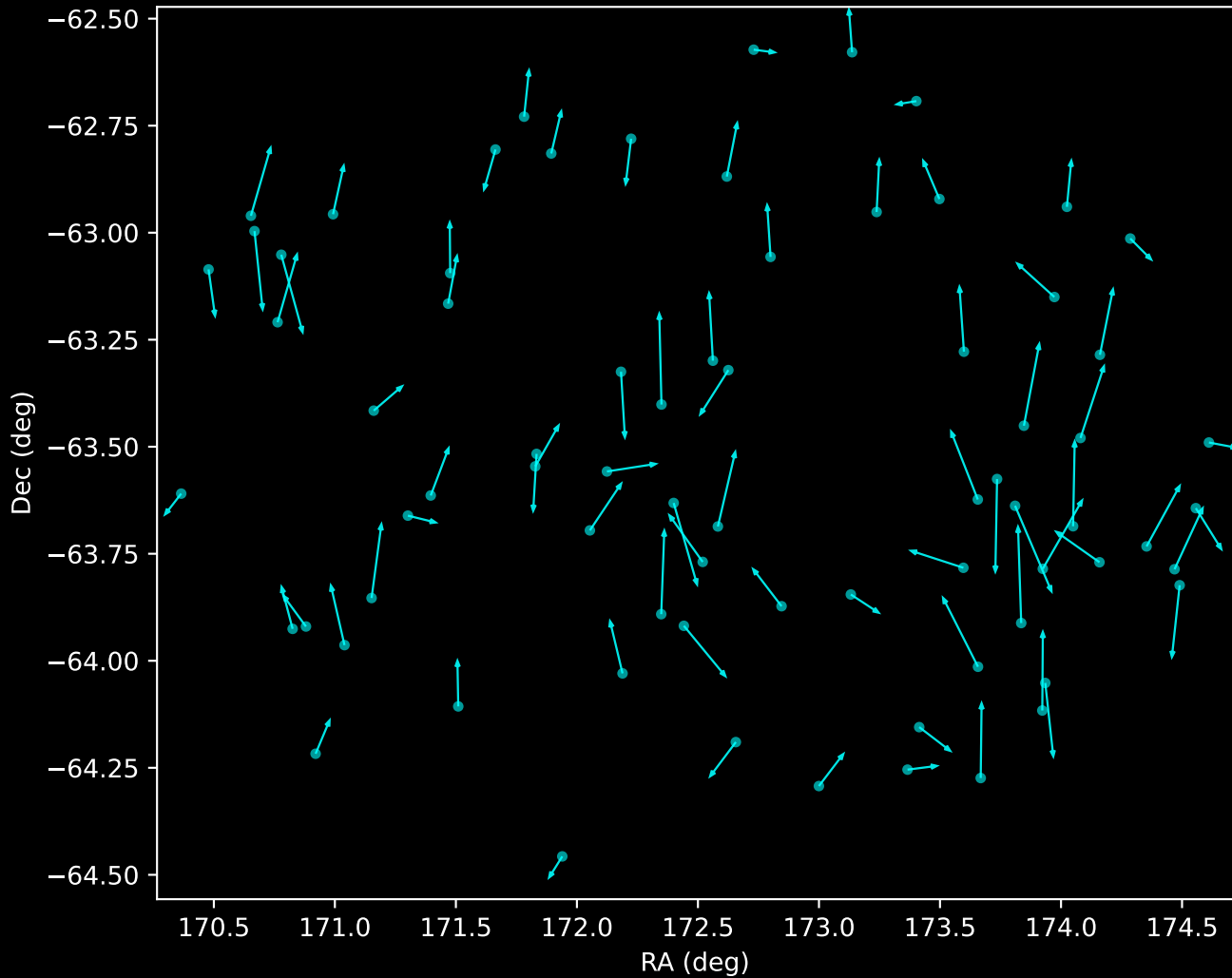
GALAH DR4 Noise Stream Proper Motion Vectors (n=74)
