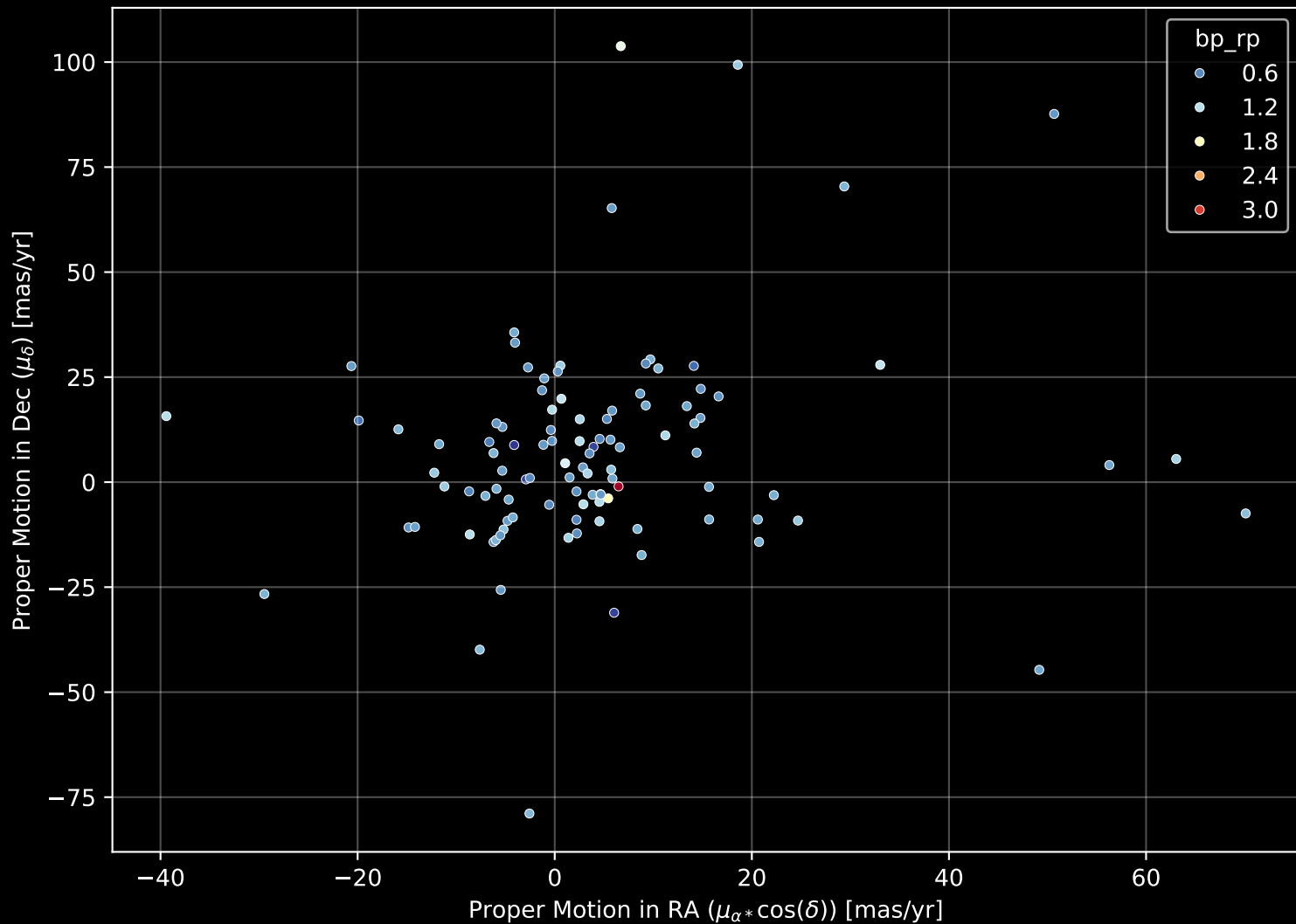
GALAH DR4 Field: [7155] Proper Motion Diagram (n= 104)
